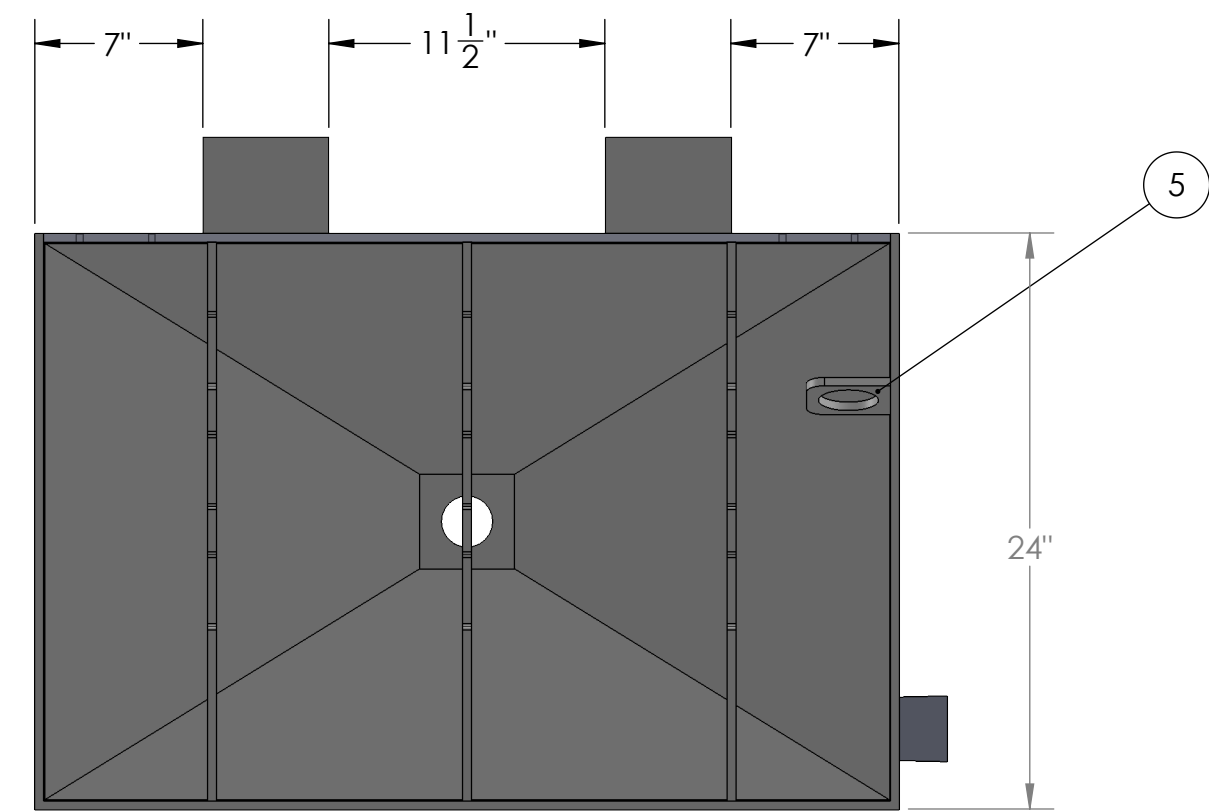
TOP PANEL TAKEN OFF FOR CLARITY
